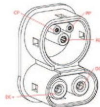
IEC62196-3: CCS Combo 2
