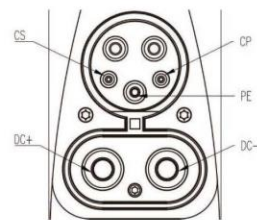
IEC62196-3: CCS Combo 1
